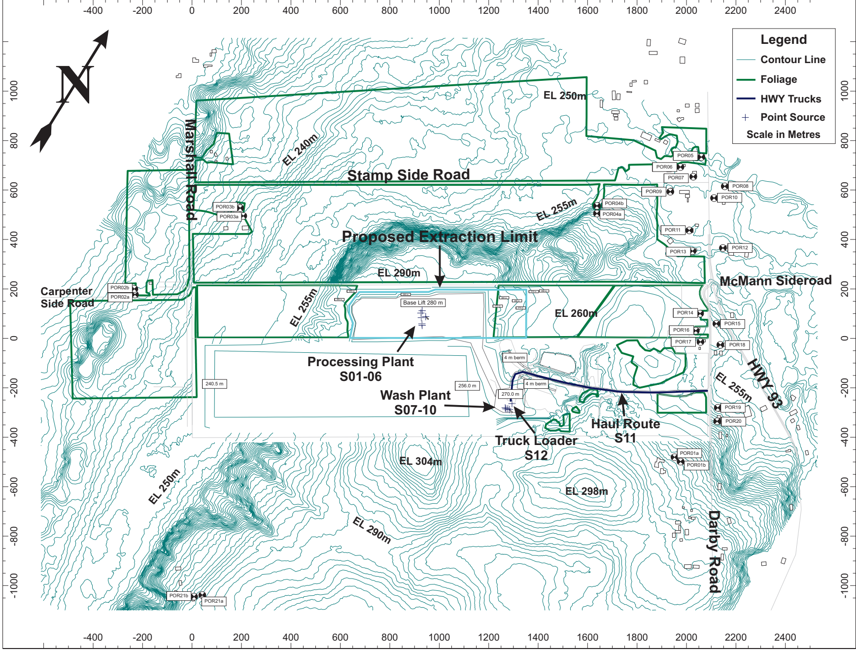
Figure 3ii: Overview of Receptor (POR) locations and Noise Source locations - Worst-Case Scenario 2
