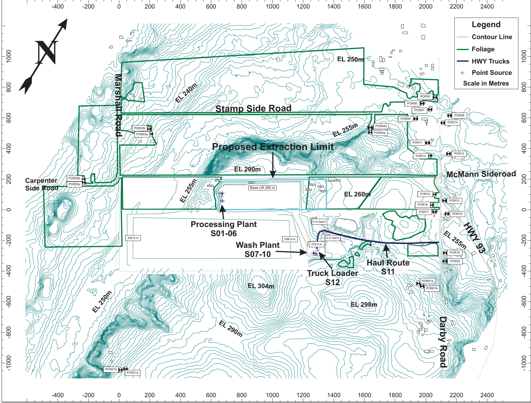
Figure 3i: Overview of Receptor (POR) locations and Noise Source locations - Worst-Case Scenario 1
